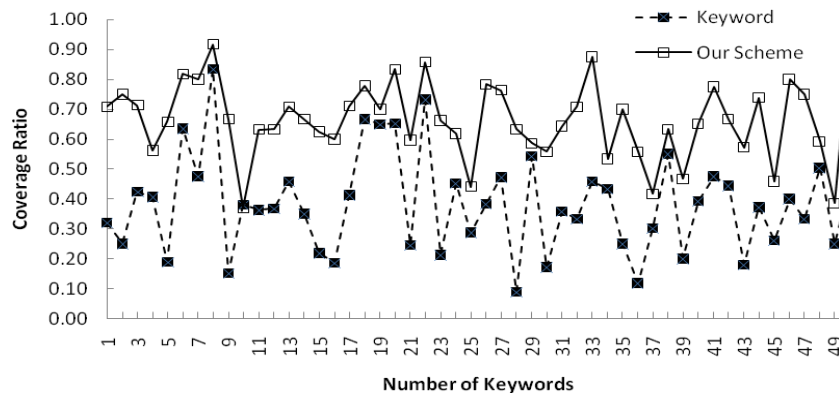
Fig. 5 comparison of the traditional Yahoo text-based search and our scheme with the ACCC algorithm
