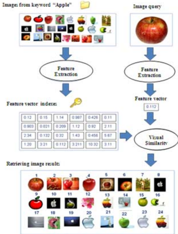
Fig. 2. A Basic principle of an on-line CBIR system
