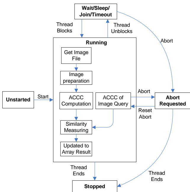
Fig. 3 The framework of multi-threaded processing for an on-line CBIR application
