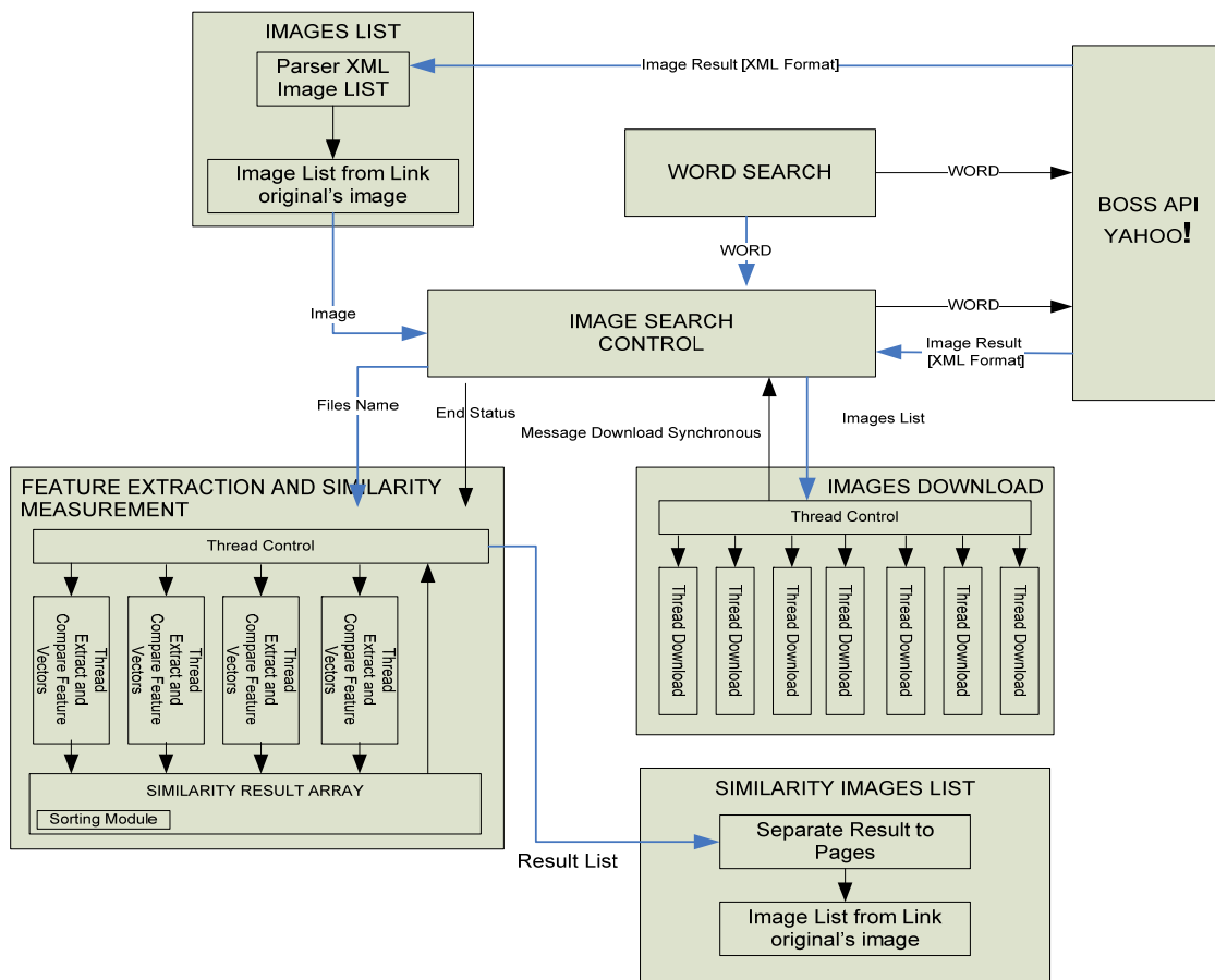
Fig. 3 The framework of multi-threaded processing for an on-line CBIR application
